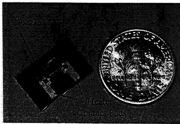
Fig. 11: Completed Vaporizing Liquid Micro-Thruster Chip
