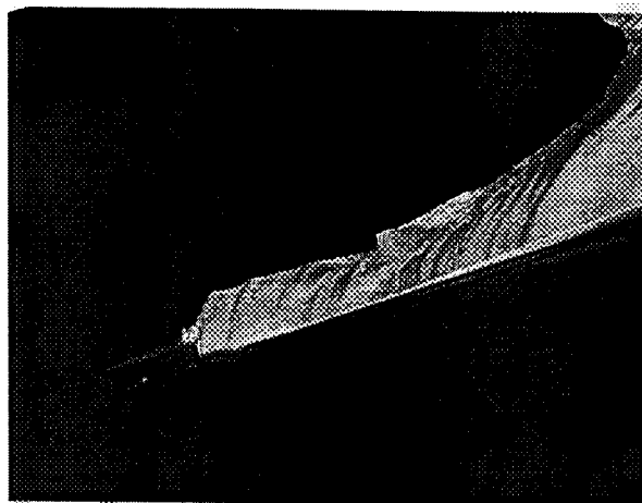
Fig. 9: Detail of Bond Width Test Chip #94 (Lower Left Corner of Fig. 8), Viewing Direction from Top of Fig. 8.
