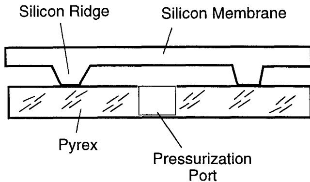
Fig. 7: Concept of Bond Width Test Chip
