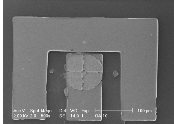
Figure 4. SEM image of the metal pattern for measurement in this study after growing nanotubes.
