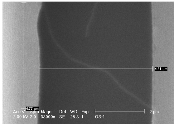
Figure 5. SEM of a CNT bridging the 4.61- \mu\text{m} gap between two electrodes at an oblique angle.
